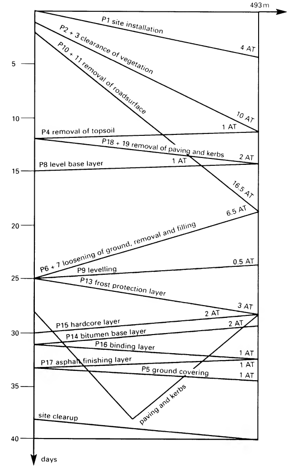
sequence of works: site installation and clearing demolition and earthworks construction of road profile metalling, paving and kerbs
